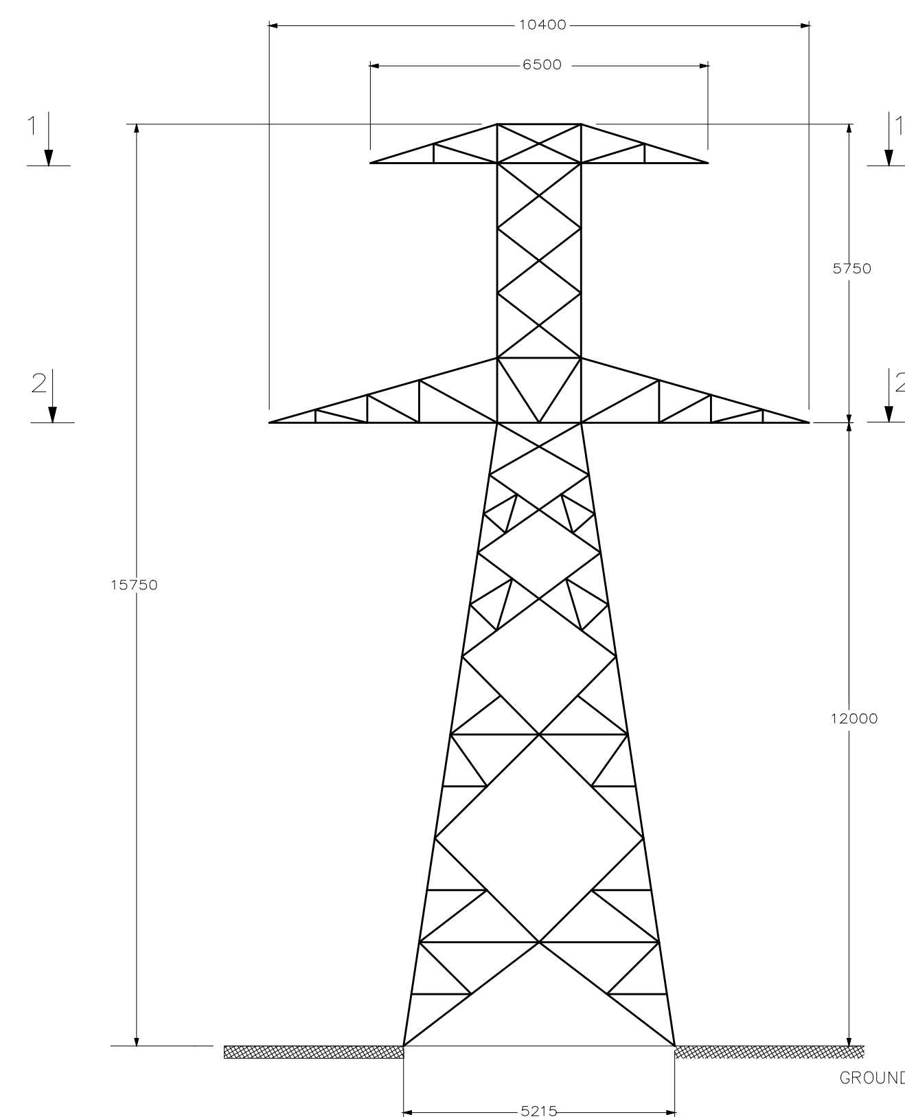
TYPICAL TRANSVERSAL FACE
