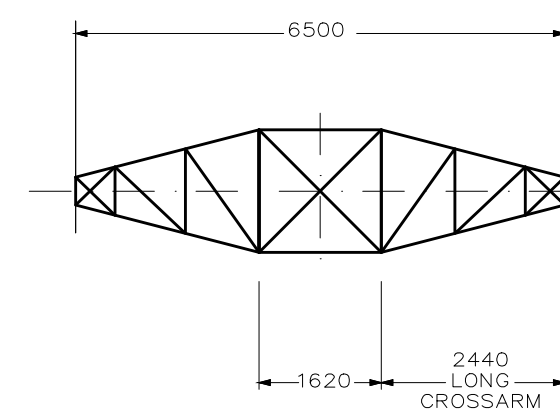
SECTION 1 - 1
