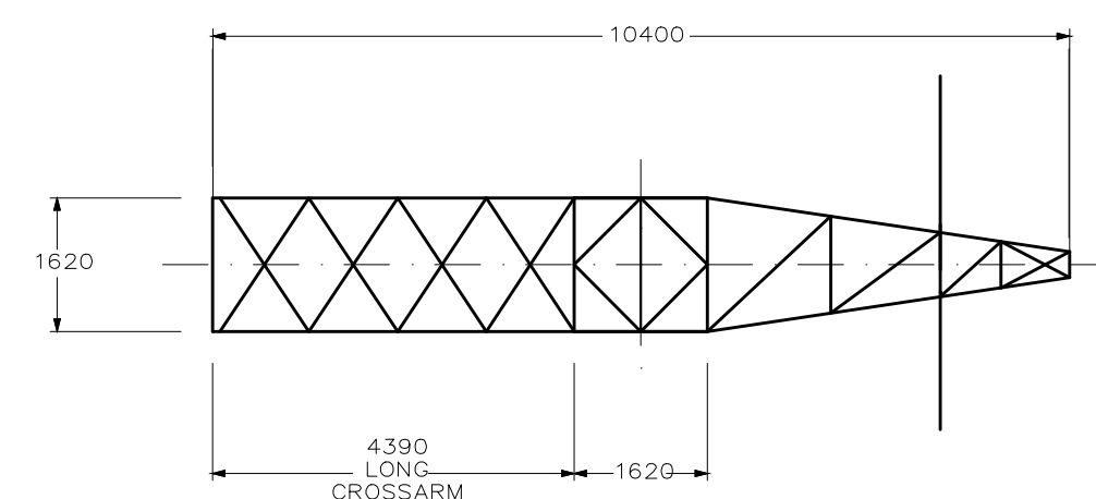
SECTION 2 - 2
